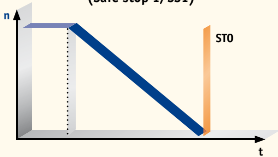
Sicherer Stopp 1 (Safe stop 1, SS1)
