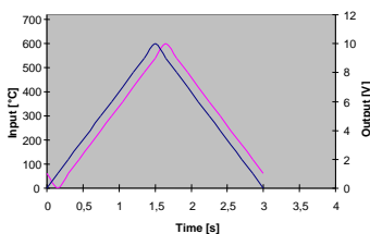
Delay of the input filter 0-600 degree
