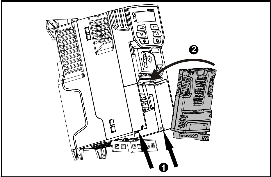
Figure 3-1 Installation of an SI option module on SIGMATEK FDD3 (sizes 2 to 4)
