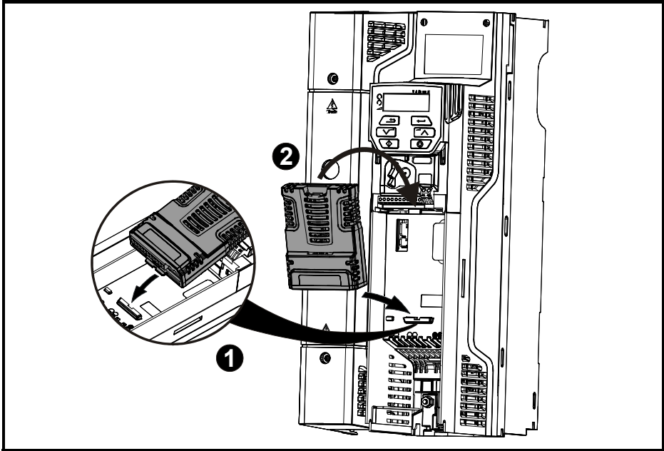
Figure 3-1 Installation of an SI option module on SIGMATEK FDD3 (size 5 to 9)
