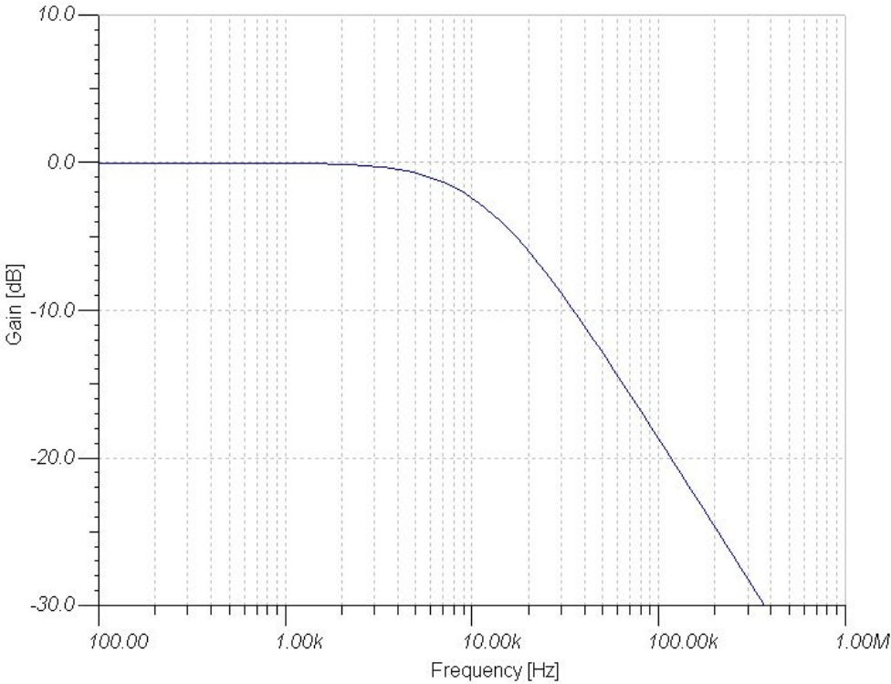
Typical differential mode frequency response
