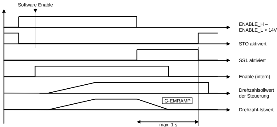
Timing Diagramm
