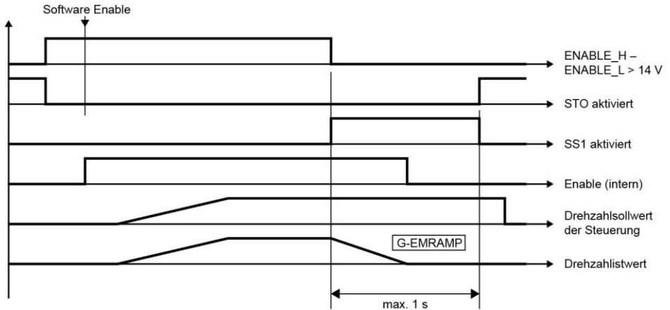
Timing Diagramm
