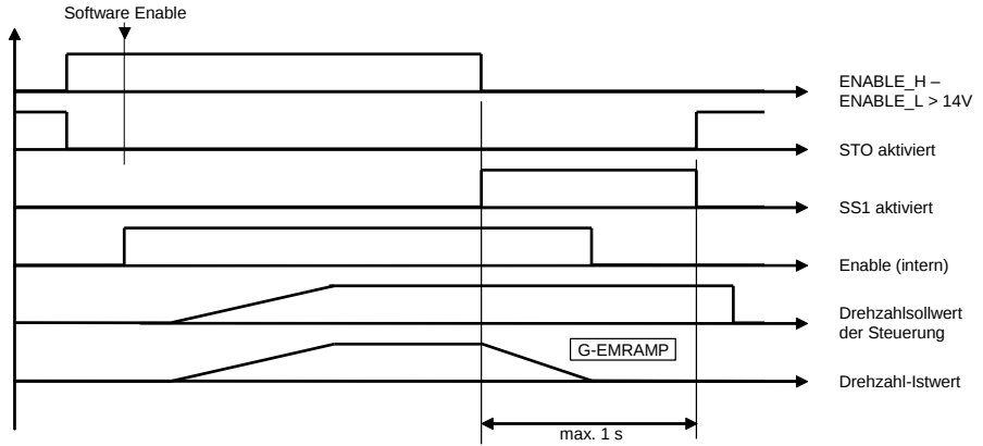
Timing Diagramm
