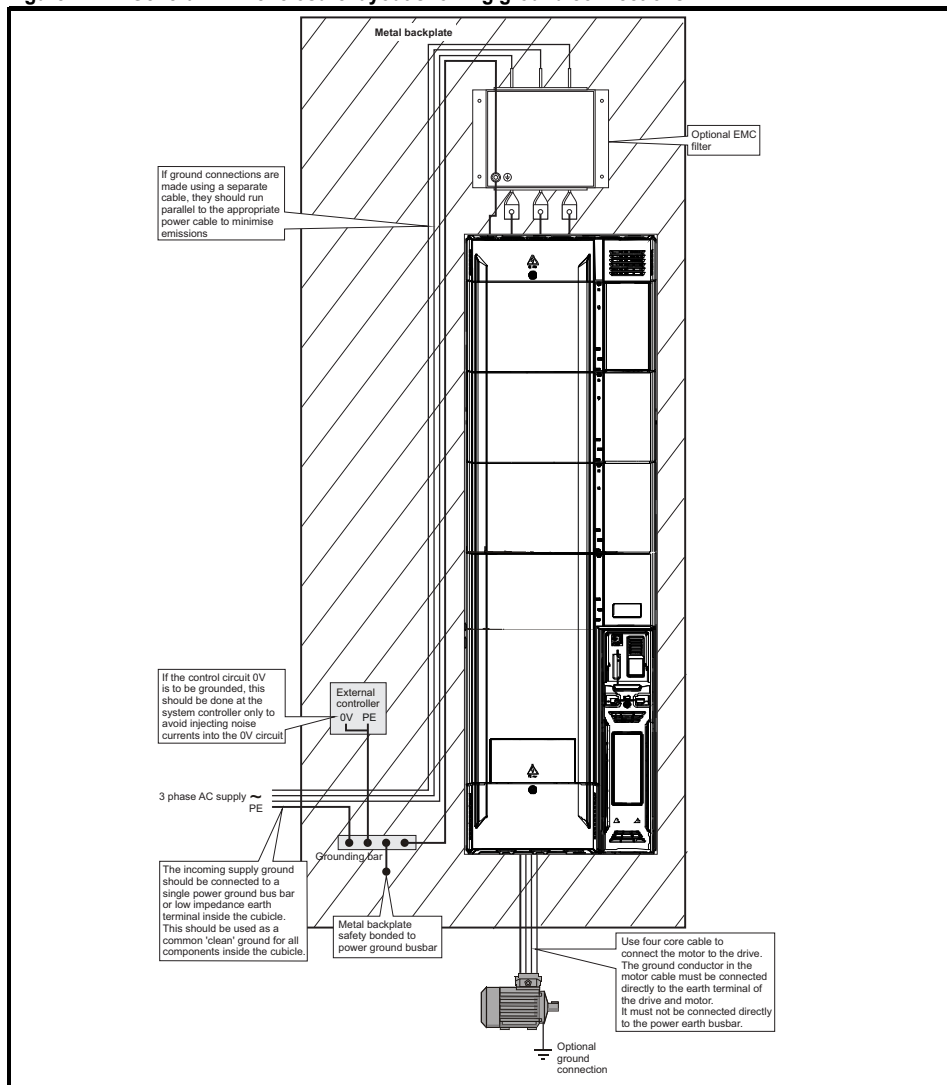
Figure 4-12 General EMC enclosure layout showing ground connections
