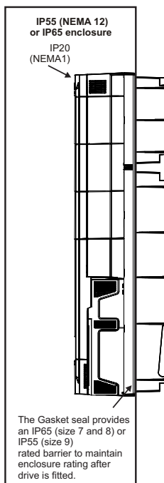
Figure 3-15 Example of high IP through-panel layout
