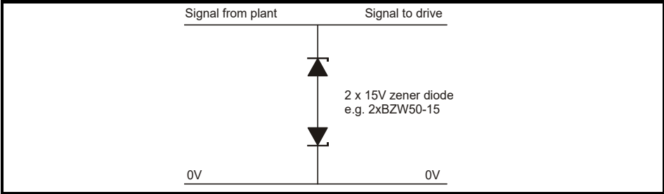
Figure 4-25 Surge suppression for analog and bipolar inputs and outputs
