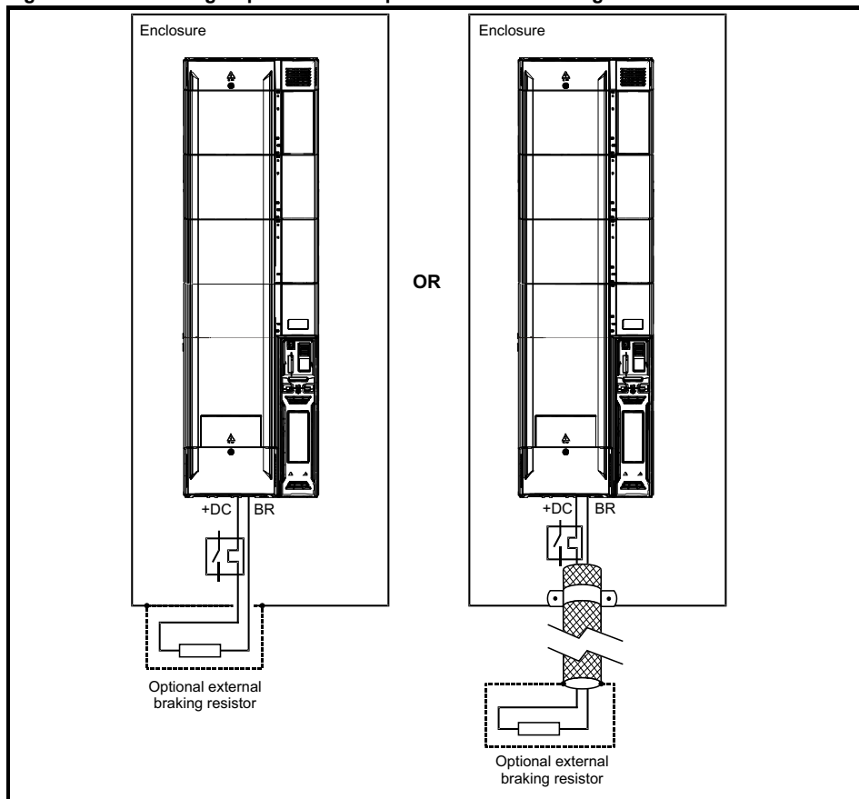
Figure 4-20 Shielding requirements of optional external braking resistor
