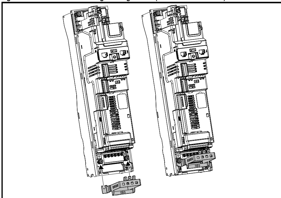
Figure 4-9 Installation of control grounding bracket (all sizes - size 3 shown)
