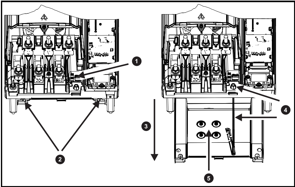
Figure 3-23 Size 9 heatsink fan replacement
