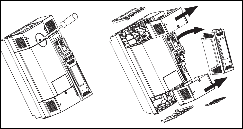
Figure 3-4 Removing the size 7 to 9 terminal covers (Size 7 shown)
