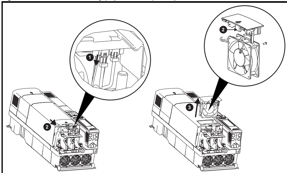
Figure 3-24 Size 7 to 9 auxiliary (capacitor bank) fan replacement
