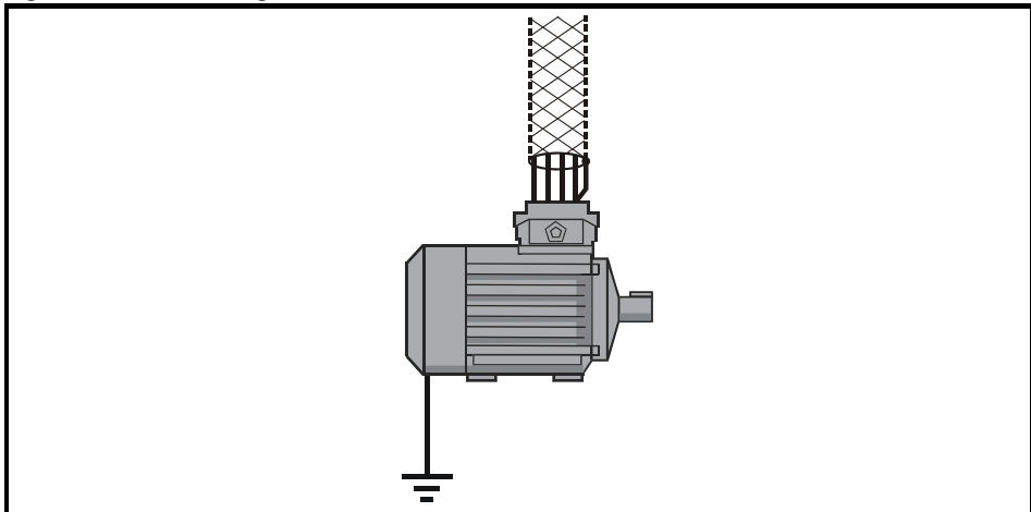
Figure 4-19 Grounding the motor cable shield
