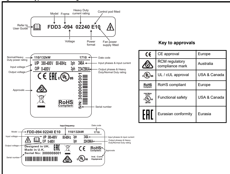
Figure 2-2 Typical drive rating labels
