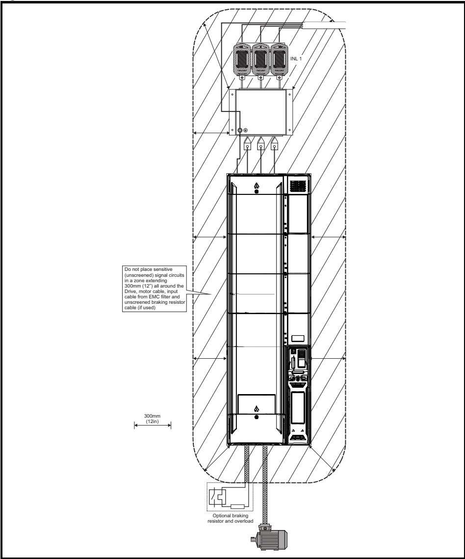
Figure 4-13 Drive cable clearances
