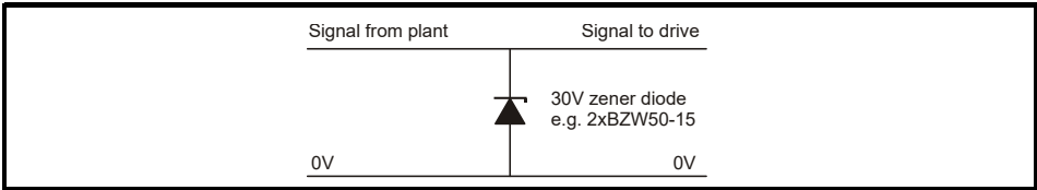
Figure 4-25 Surge suppression for analog and bipolar inputs and outputs
