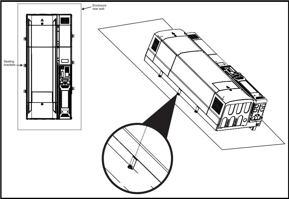
Figure 3-16 View showing sealing clamps provided in through hole mounting kit
