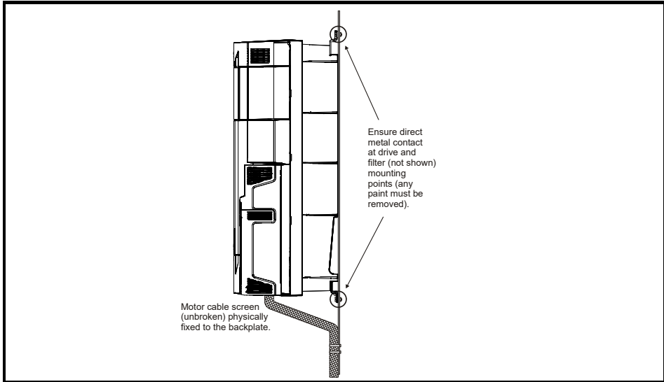
Figure 4-18 Grounding the drive, motor cable shield and filter
