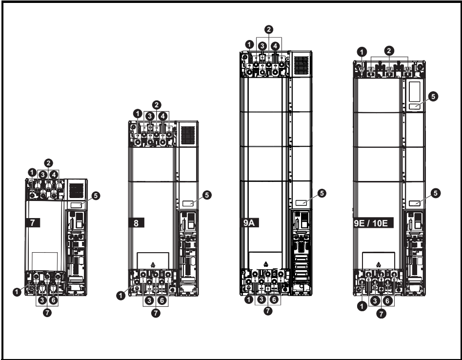
Figure 2-3 Features of the drive (size 7 to 9)
