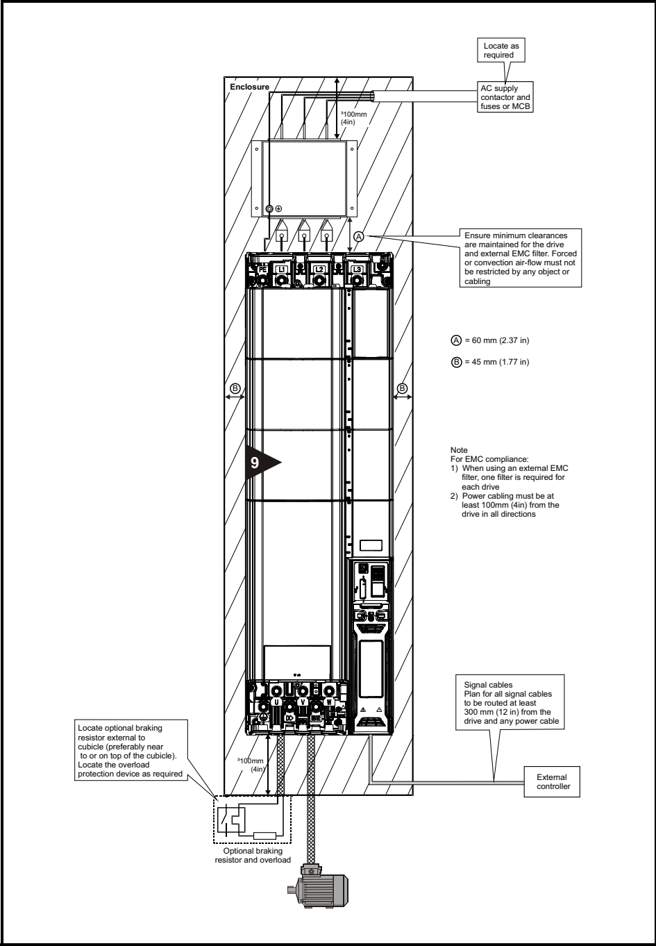
Figure 3-11 Enclosure layout (size 9)
