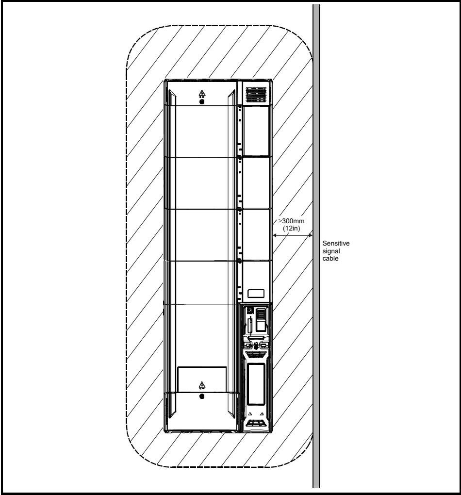
Figure 4-17 Sensitive signal circuit clearance
