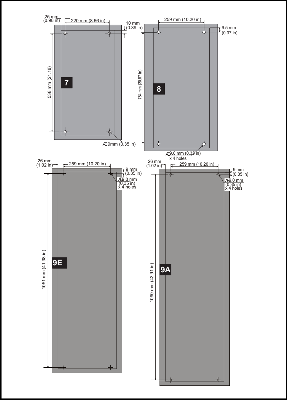
Figure 3-7 Surface mounting dimensions (size 7 to 9)
