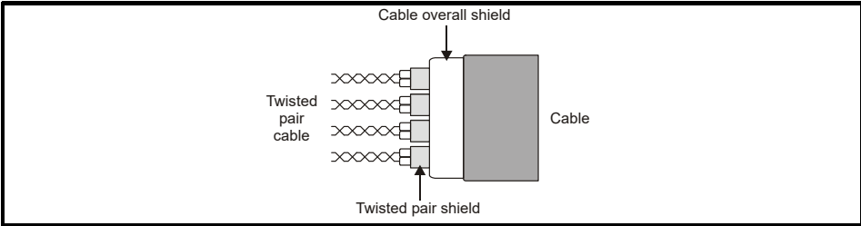
Figure 4-15 Feedback cable connections
