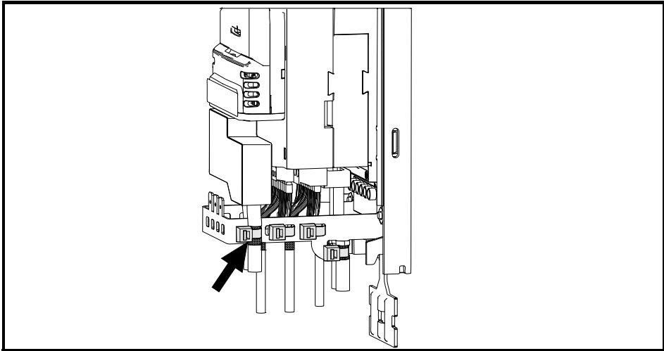
Figure 4-21 Grounding of signal cable shields using the grounding bracket
