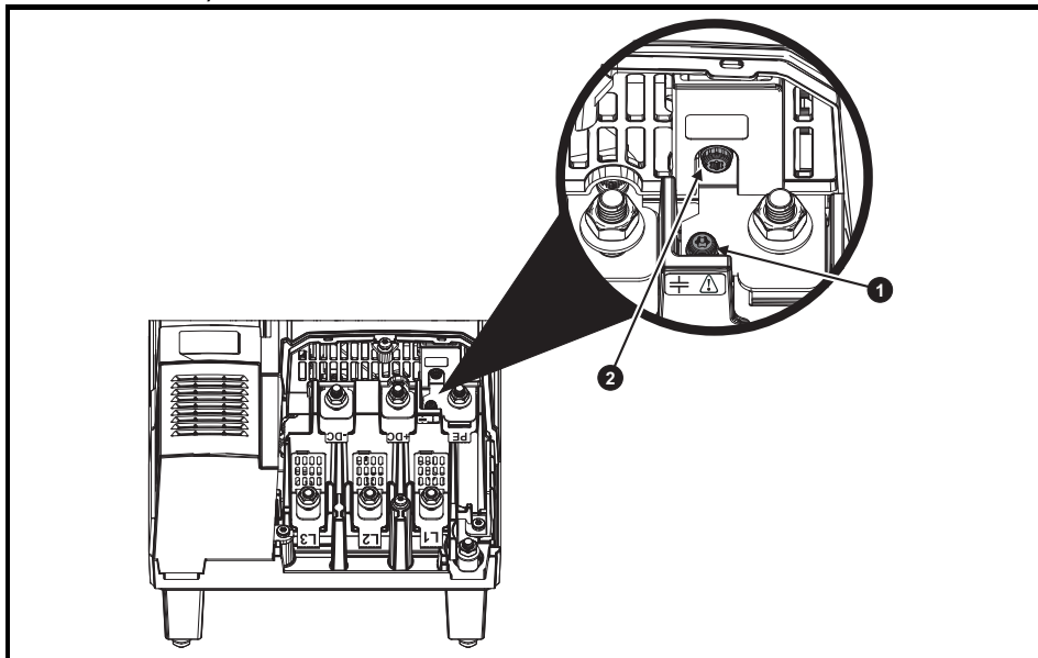
Figure 4-10 Removal of the size 7, 8 and 9A internal EMC filter and line to ground varistors (size 7 shown)
