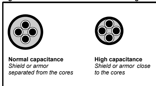
Figure 4-5 Cable construction influencing the capacitance
