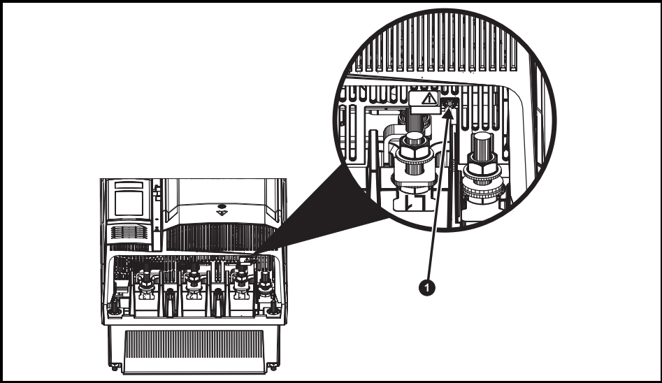
Figure 4-11 Removal of size 9E line to ground varistors
