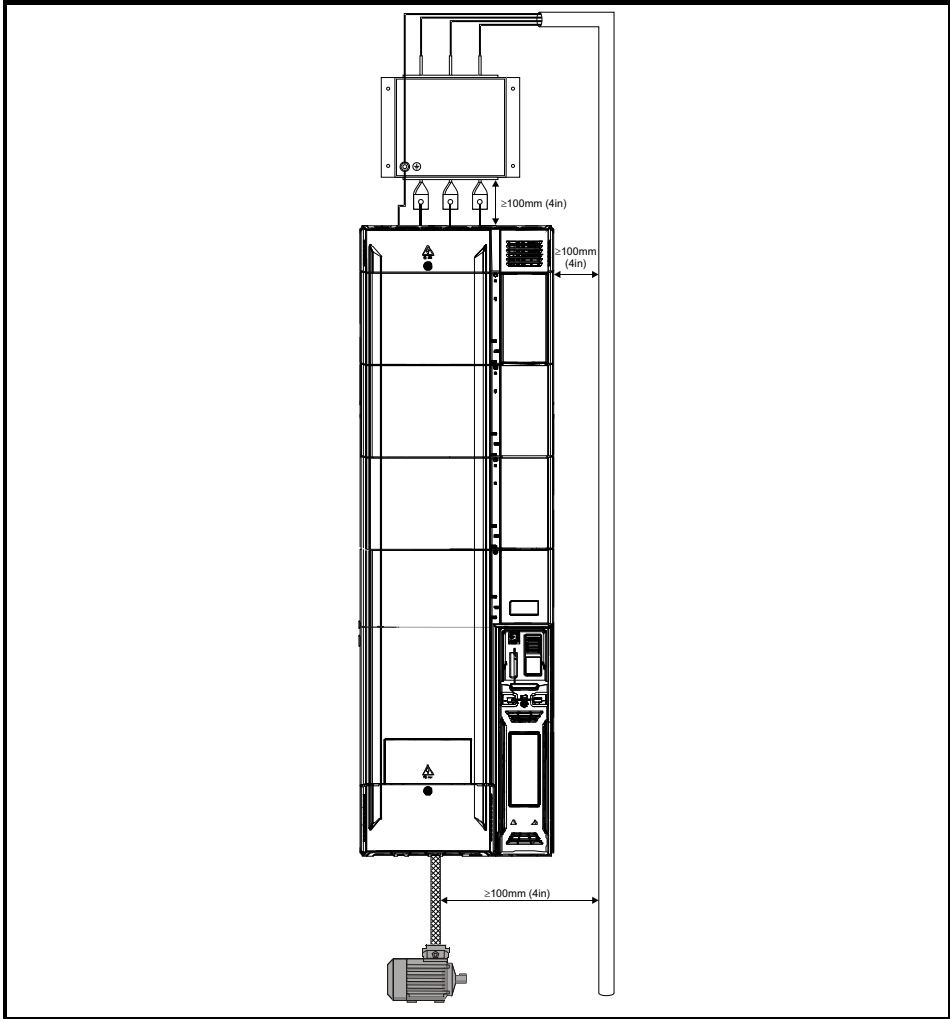
Figure 4-16 Supply and ground cable clearance
