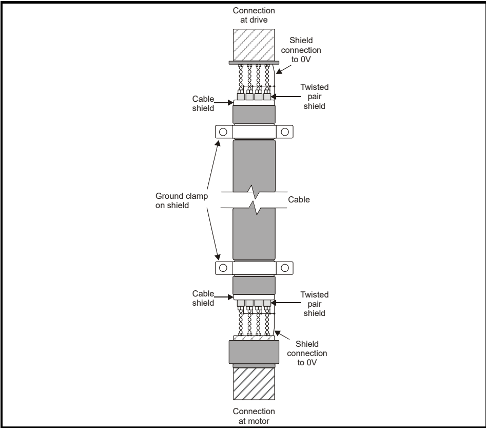
Figure 4-15 Feedback cable connections
