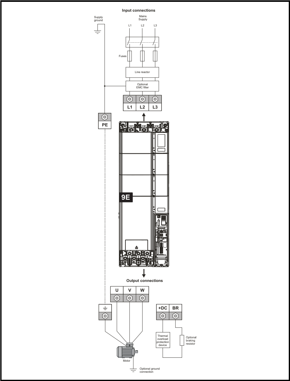
Figure 4-3 Size 9E power and ground connections
