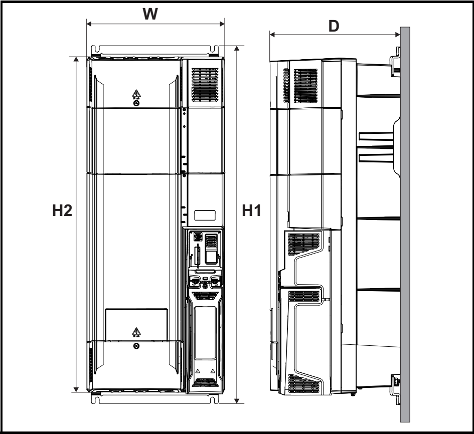
Figure 3-6 Drive dimensions (Size 8 shown)
