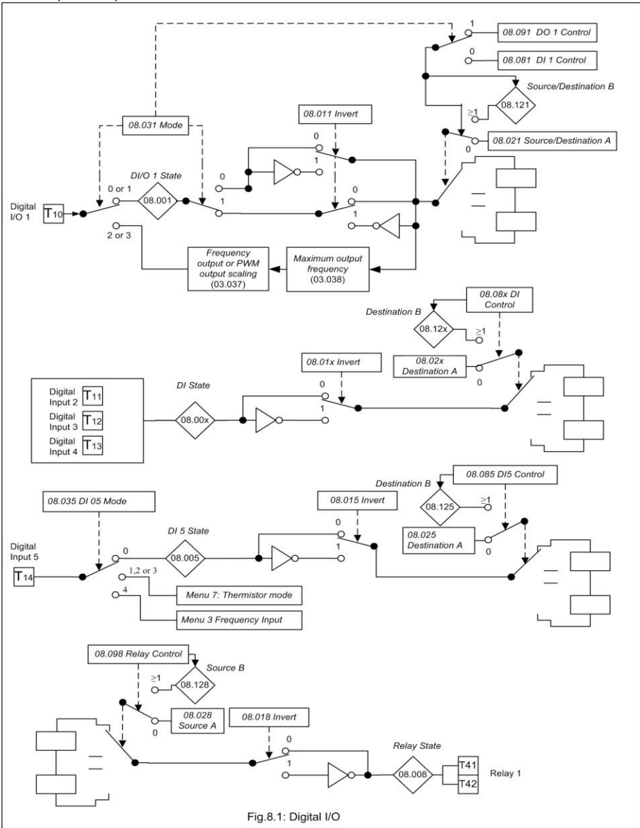
Fig.8.1: Digital I/O
