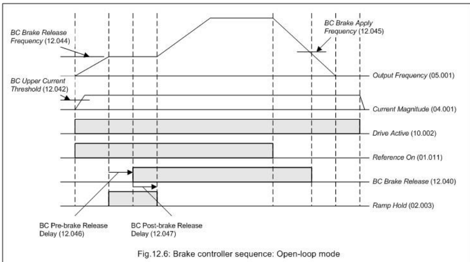
Fig.12.6: Brake controller sequence: Open-loop mode
