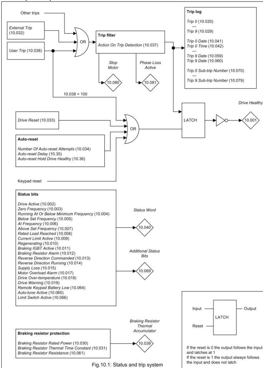
Fig. 10.1: Status and trip system
