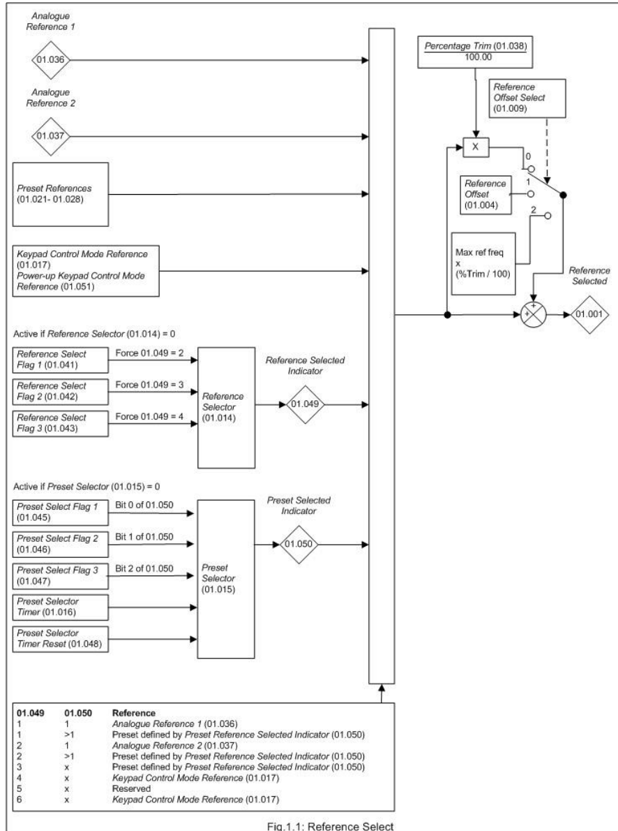
Fig.1.1: Reference Select
