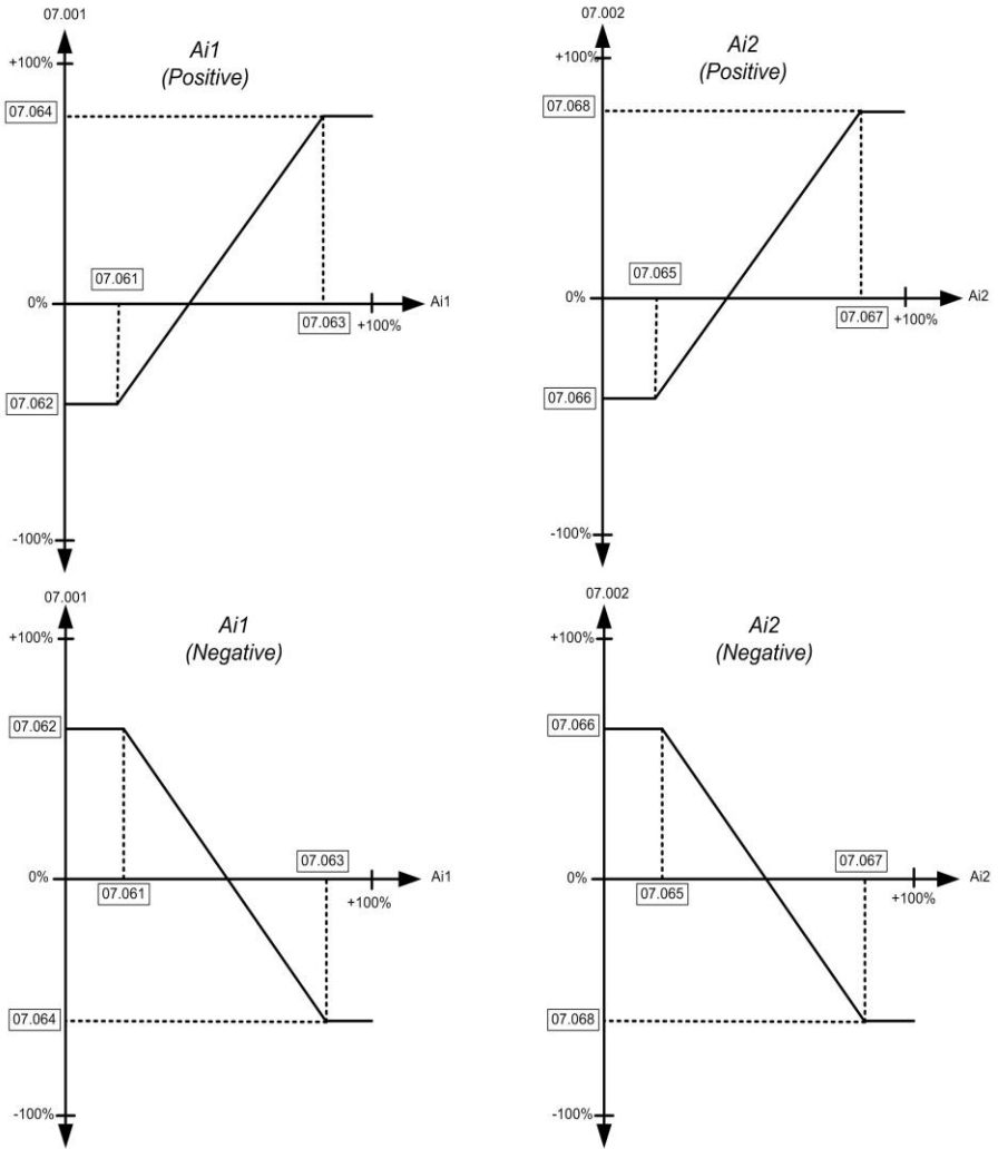
Fig.7.5b: Analog Input scaling & limit
