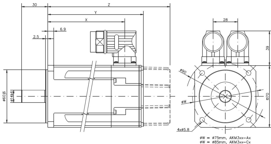
Option Keyway
