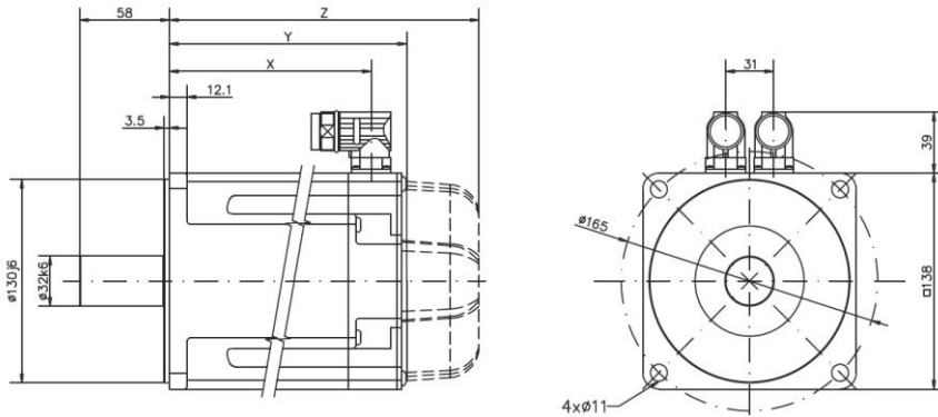
Option Keyway
